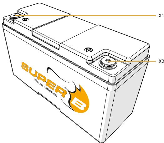
Figure 2. Connections
